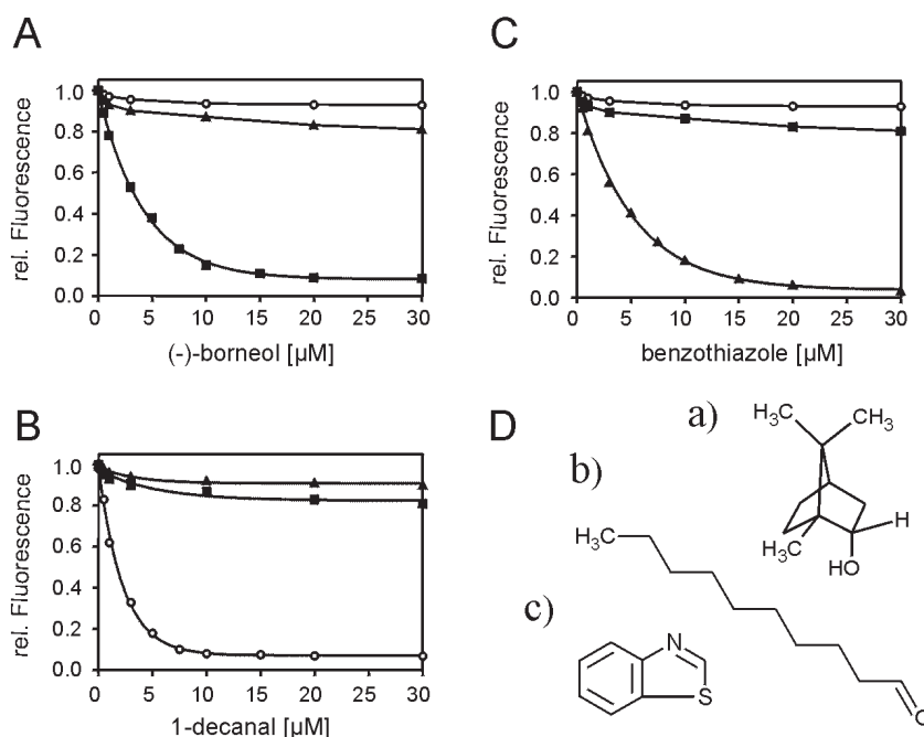
Figure 2 Selective competition of chromophore binding by odorants. Fluorescence of 2 \mu\text{M} pre-equilibrated OBP–chromophore complex was assumed as 1 for OBP1–1-AMA (filled squares), OBP2–1,8-ANS (open circles) and OBP3–1-AMA (filled triangle). Spectra were recorded at 25°C with an excitation wavelength of 256 nm. (A) Selective decrease of fluorescence intensity upon titration with (–)-borneol (a) was only observed for OBP1–1-AMA. (B) Loss of fluorescence intensity by increasing concentration of 1-decanal (b) was obtained for the complex OBP2–1,8-ANS. (C) Decrease of fluorescence upon titration with benzothiazole (c) selectively for OBP3–1-AMA. (D) Chemical structure of the odorants used in the competition experiments (a–c).
